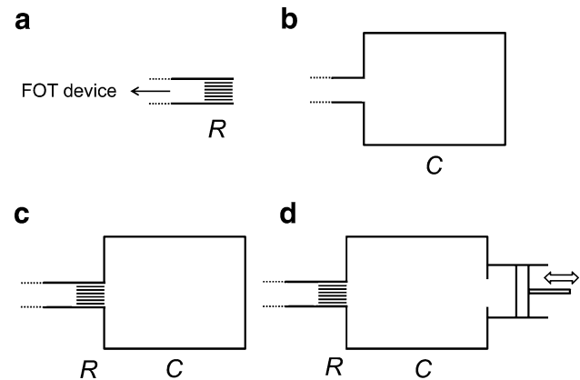
Fig. 1 Schema for four phantom models. a R model. b C model. c RC model. d RC ventilation model. R resistance using a standard resistor, C air compliance using a wooden box of known volume
