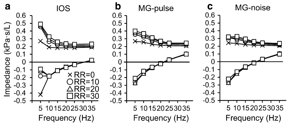
Fig. 4 Comparison of impedance values in the RC model (resistance of 0.196 kPa s/l and C model-1) measured with IOS, MG-pulse, and MG-noise. Plotted data are the mean values of three measurements
